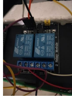
Gambar 1. 7 Relay
