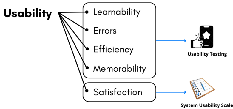
Gambar 4. Metode Penelitian
