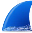
Gambar II.1 Logo Wireshark
