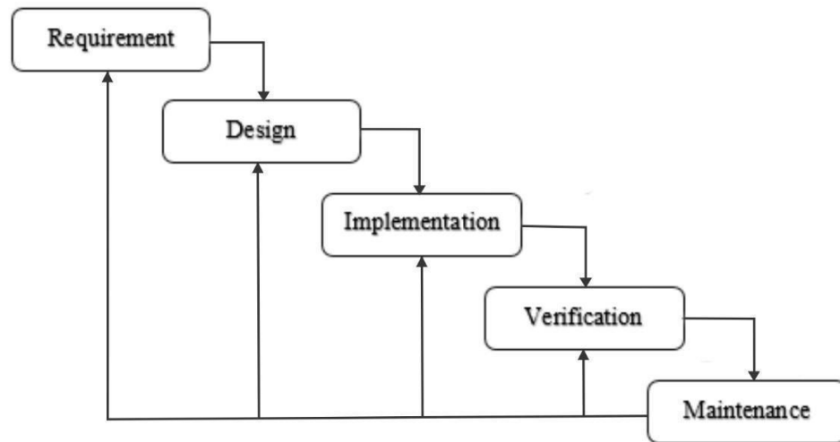
Gambar 1-1 Metodologi Waterfall
