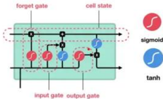
GAMBAR 2.4 DIAGRAM STRUKTUR LSTM [19]
