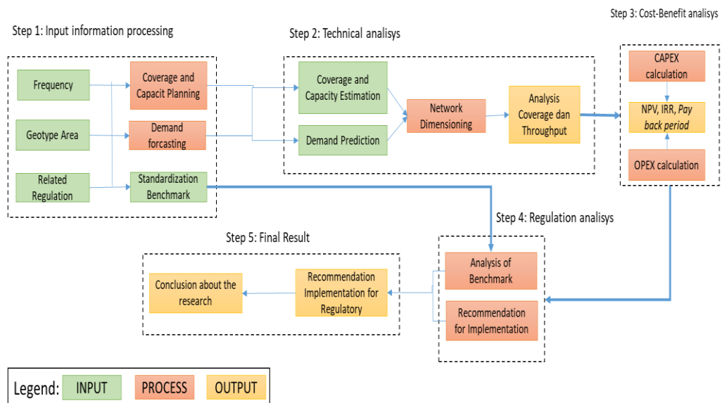
Figure 1. 2 Methodology Scheme
