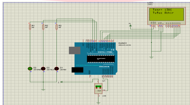
Gambar 4 Perancangan Hardware
