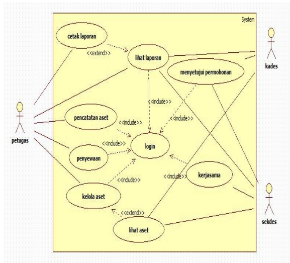
Gambar 10. Usecase Diagram Usulan
