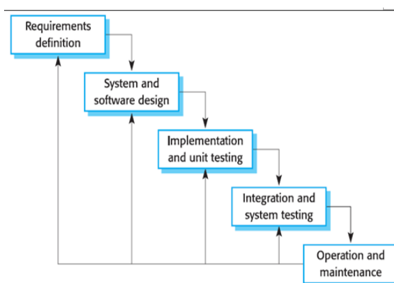
Gambar 1. Model Waterfall [1]
