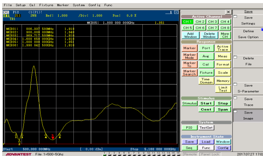
Gambar 4.1 Gambar VSWR
