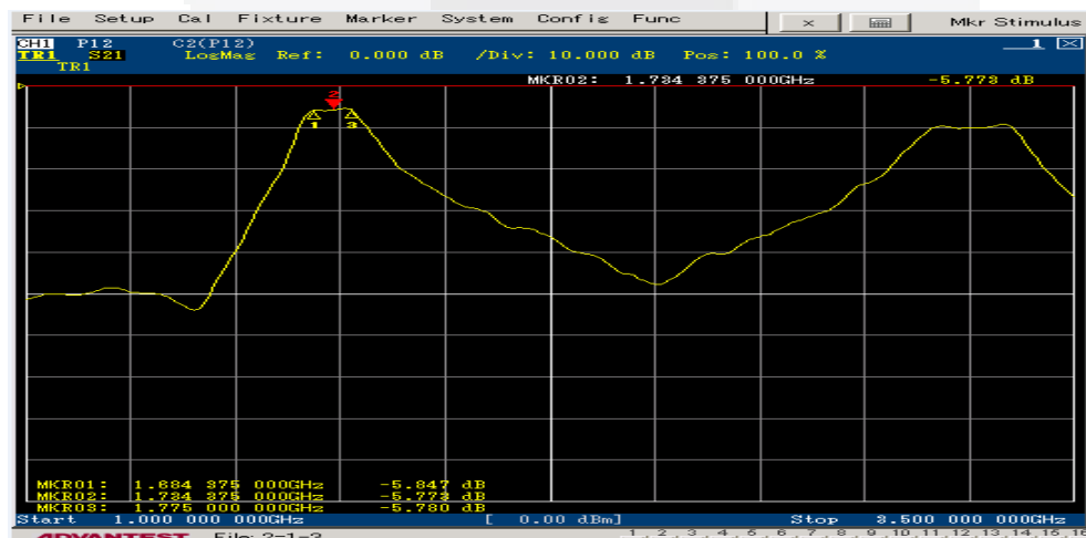
Gambar 4. 2 Hasil Pengukuran Insertion Loss
