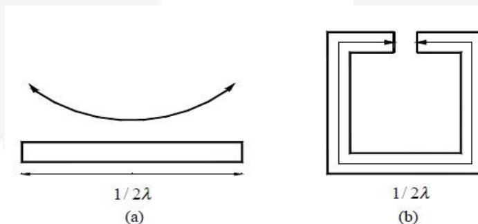
Gambar 2. 1 Struktur Square Loop Resonator [2]
