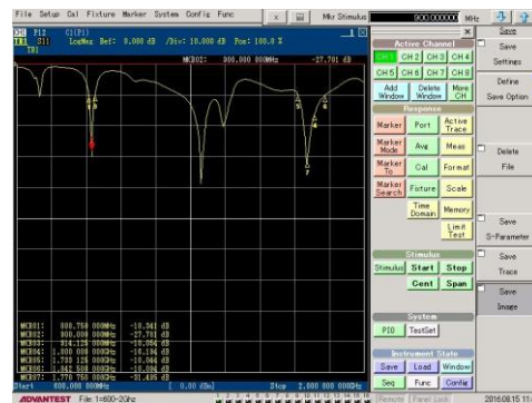
Gambar 5 Return Loss Antena
