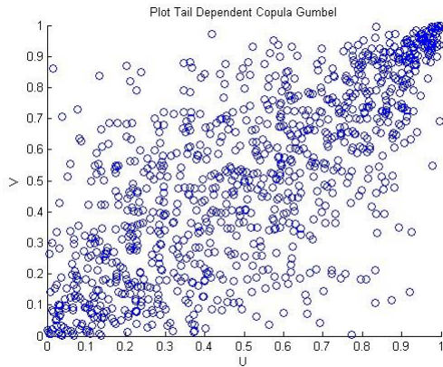
Figure 7: Scatterhist Perilaku Tail Dependence Copula Gumbel
