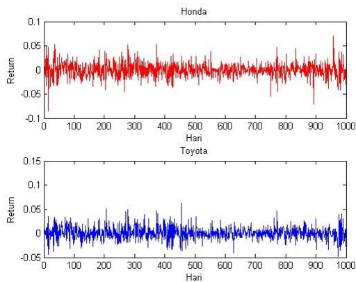
Figure 3: Nilai return Honda dan Toyota
