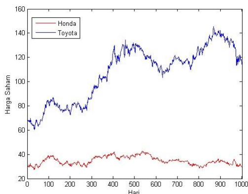
Figure 1: Harga Penutupan Saham Honda dan Toyota
