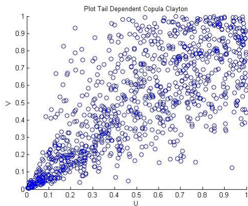
Figure 6: Scatterhist Perilaku Tail Dependence Copula Clayton
