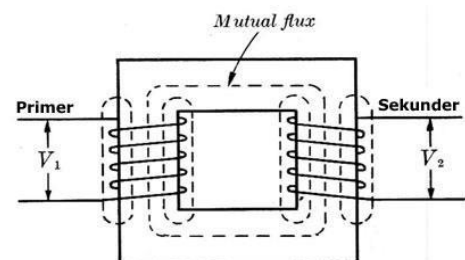
Gambar 1 Transformator
