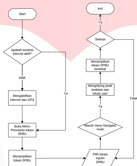
Gambar 4.1 Flowchart system
