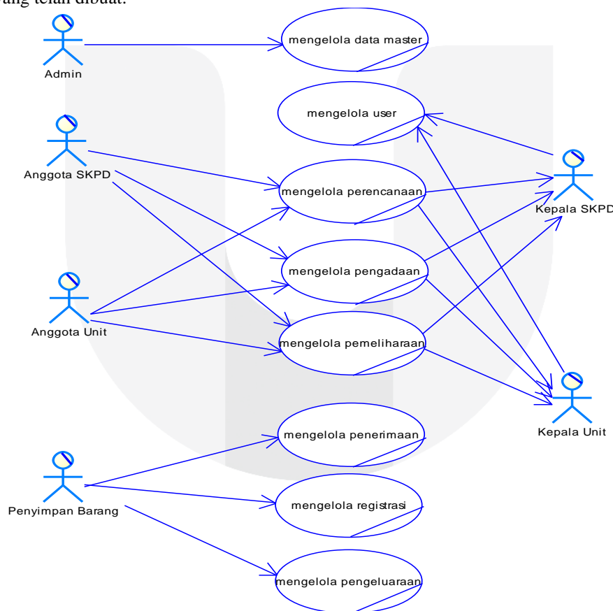
Gambar 2. Bussiness Use Case Diagram
