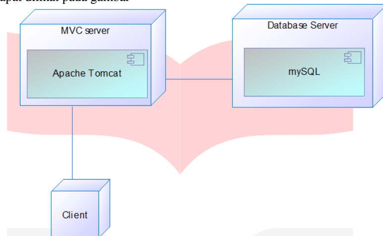
Gambar 3 Deployment Diagram Tahap Transisi
