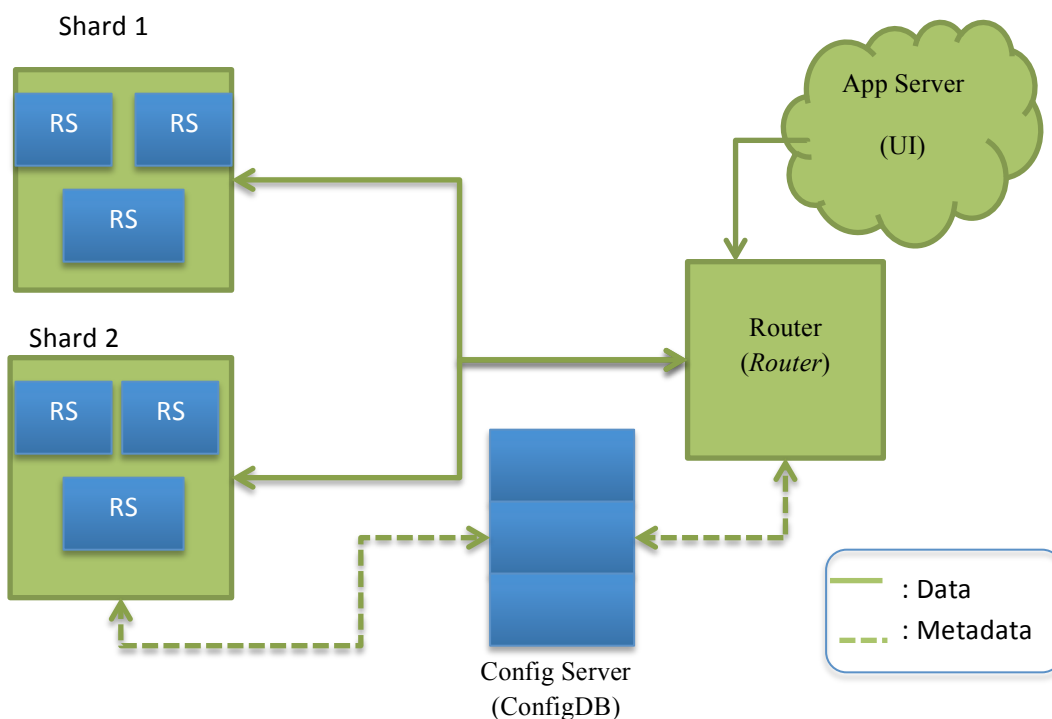
Gambar 2-3: Topologi Sharding [1]
