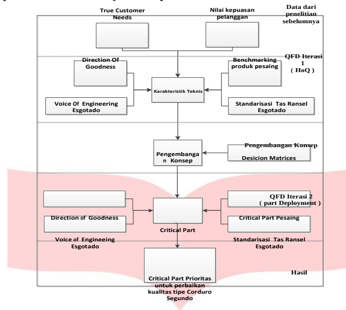
Gambar 3. Model Konseptual
