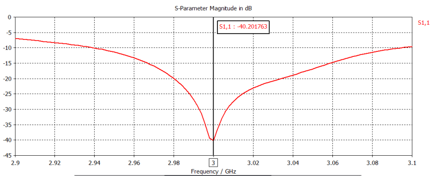
Gambar 2.5 Nilai Return Loss
