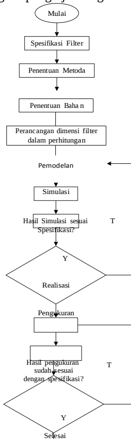
Gambar 2.4 Flowchart Sistem
