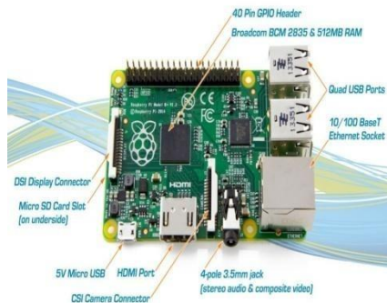
Gambar 2 Raspberry Pi Model B+
