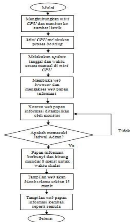
Gambar 4 Flowchart sistem tampilan jadwal adzan
