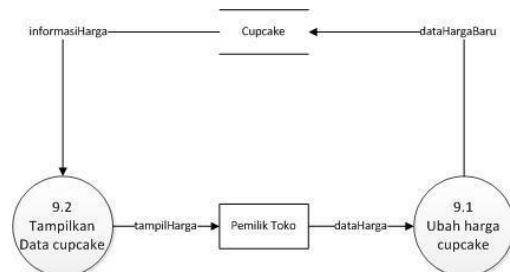
Gambar 3.20 Proses Perubahan Harga Cupcake
