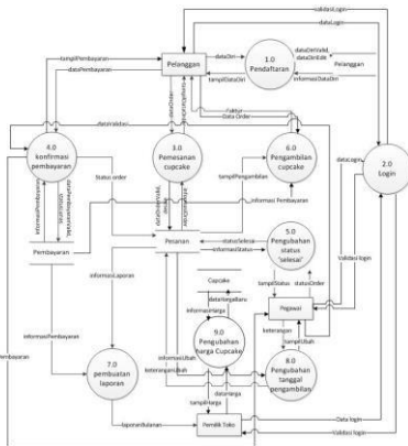
Gambar 3.14 Data Flow Diagram Level 1
